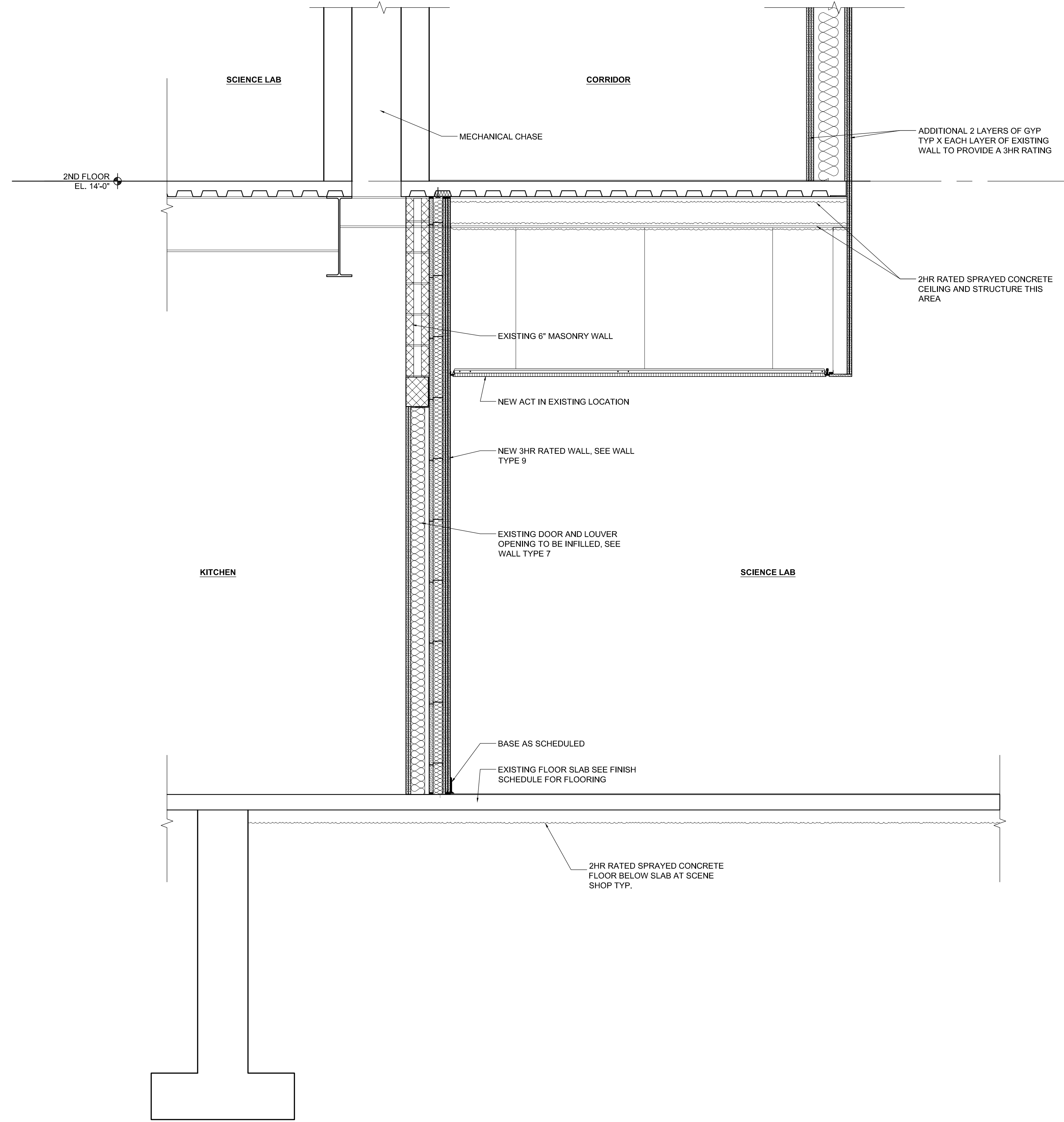
2 SECTION THRU SCENE SHOP AND KITCHEN SCALE: 3/4" = 1'-0"
