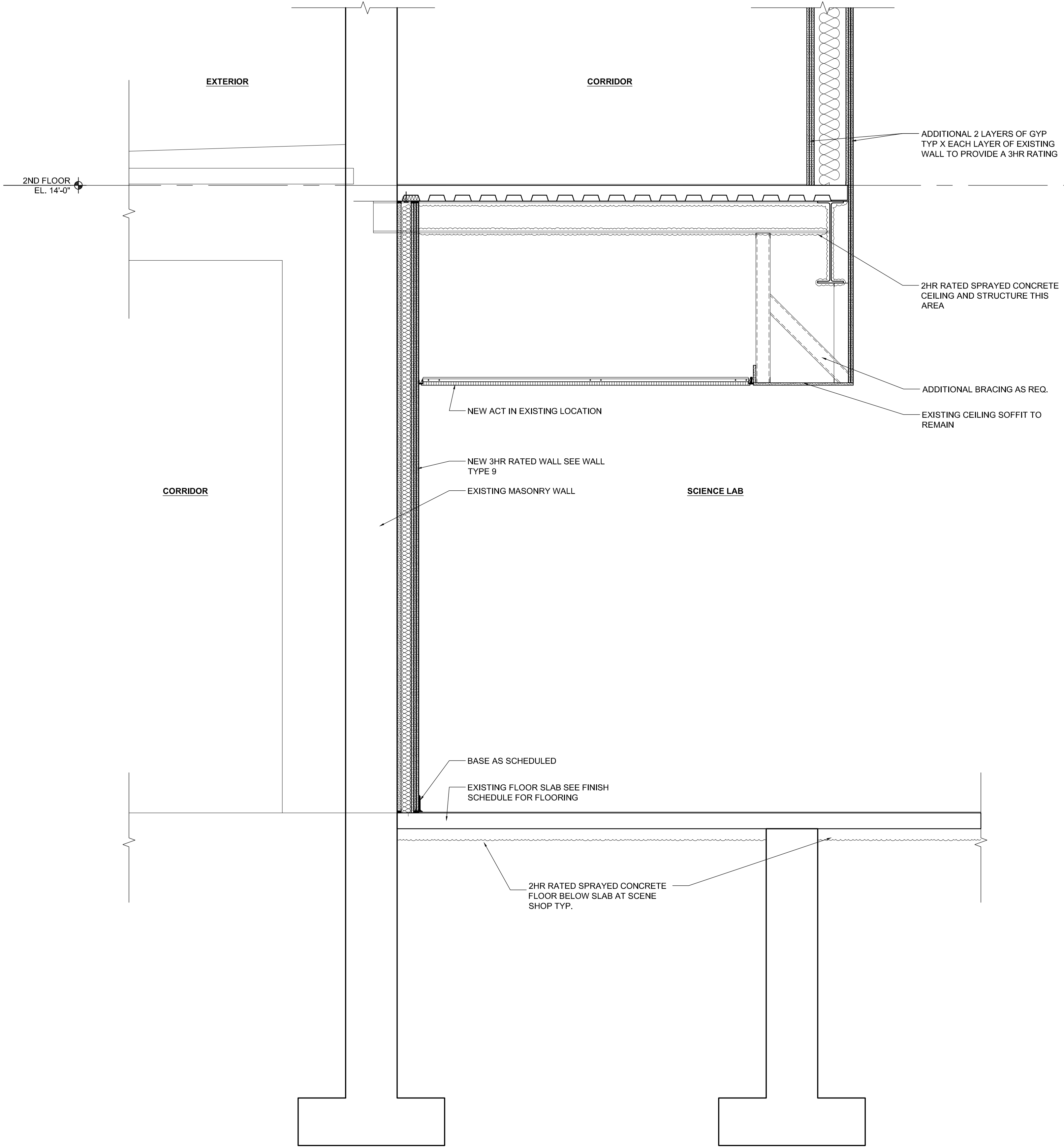
1 SECTION THRU SCENE SHOP AND CORRIDOR SCALE: 3/4" = 1'-0"
